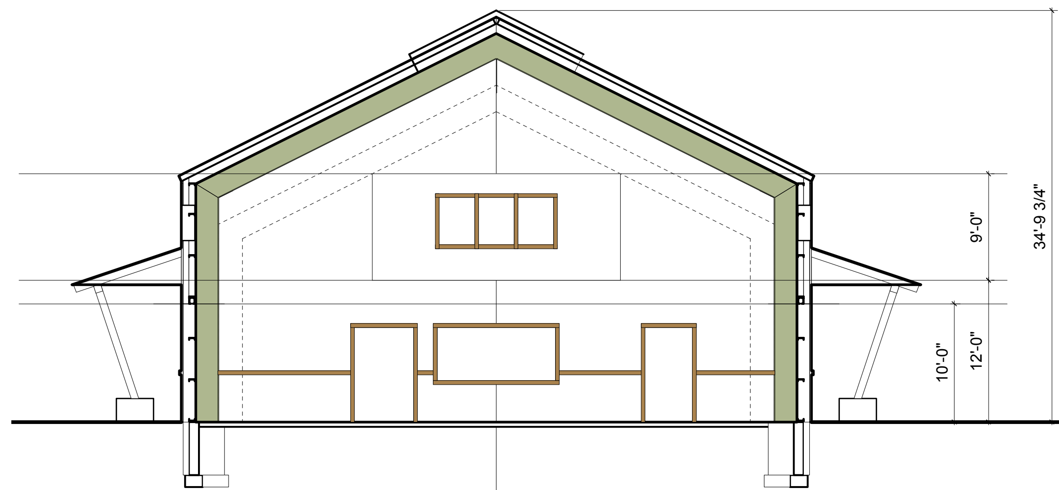
22 BUILDING SECTION Scale: 1/8" = 1'-0"
